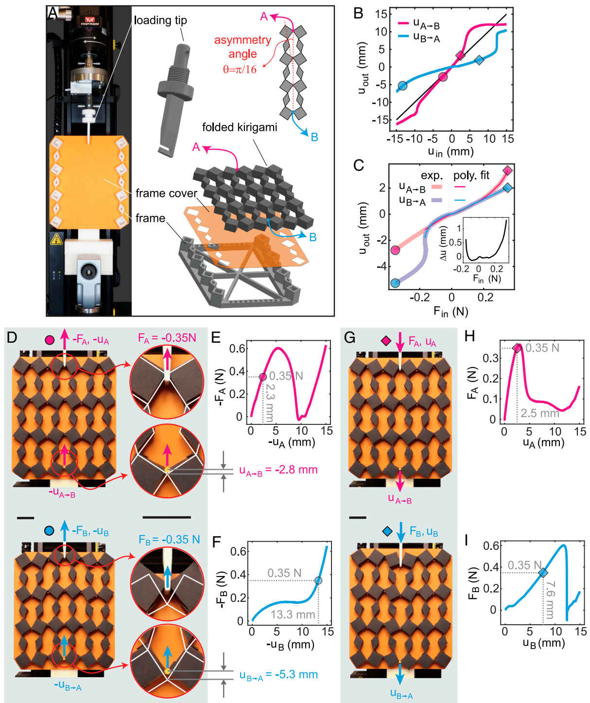
Fig. 5. Experimental validation of nonreciprocity of square-rhombus “folded kirigami”. (A) Setup for the compression and tension tests. (B) Experimental curves of output displacement u_{out} versus input displacement u_{in} for loads applied at points A (magenta) and B (blue). (C) Experimental curves (and polynomial fit) of output displacement u_{out} versus input force F_{in} loaded at points A and B, revealing nonreciprocal behavior for large deformations. Inset: Nonreciprocal measurement \Delta u = u_{A \rightarrow B} - u_{B \rightarrow A} , obtained by plotting the difference of the two polynomials. (D) Snapshots showing lattice deformations for tensile loads applied at points A (magenta) and B (blue). (Scale bars, 3 cm.) (E and F) Force–displacement curves for tensile loads. (G) Snapshots showing lattice deformations for compressive loads applied at points A (magenta) and B (blue). (Scale bars, 3 cm.) (H and I) Force–displacement curves for compressive loads.
